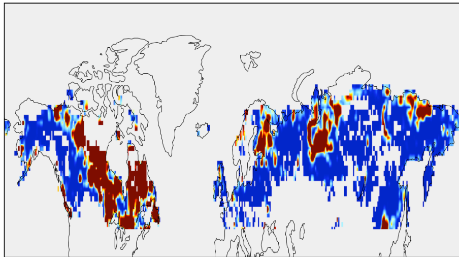
(a) Satellite observed flooded areas (non frozen)
