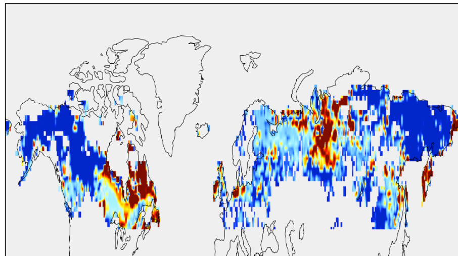
(b) Modelled flooded peatland
