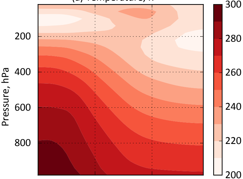
(a) Temperature, K
