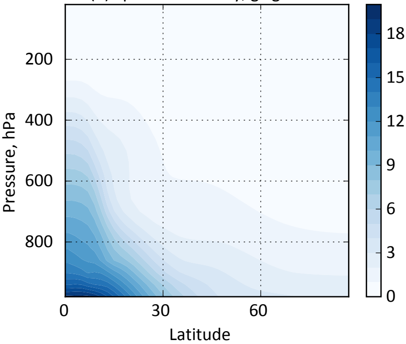
(b) Specific humidity, \text{g kg}^{-1}
