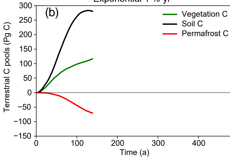
Exponential 1 % yr -1
