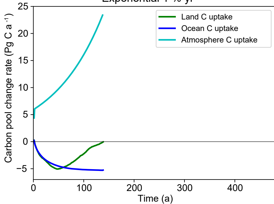
Exponential 1 % yr -1
