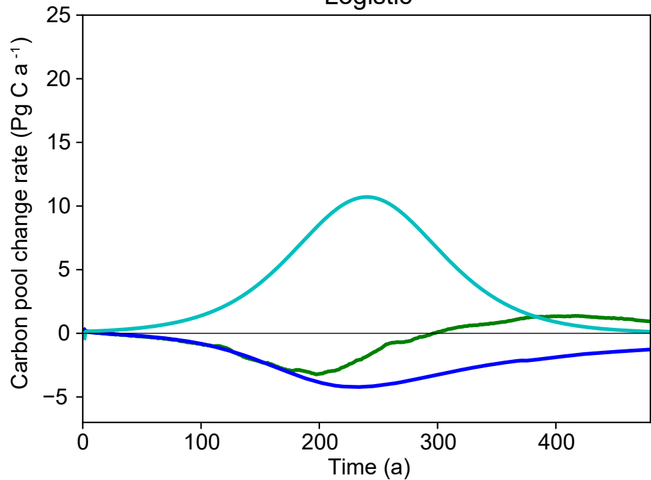
Logistic
