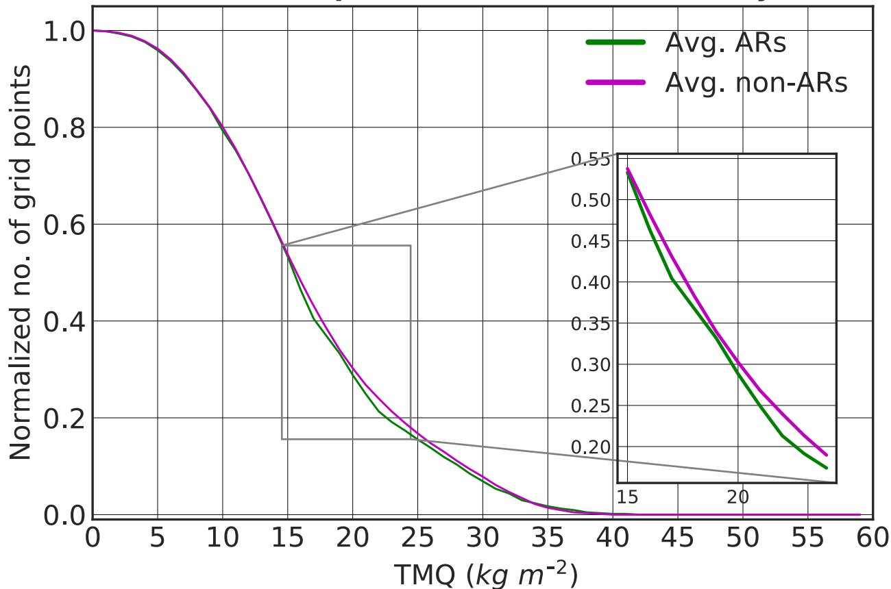
Evolution plot - CAM5.1 (200 km; daily)
