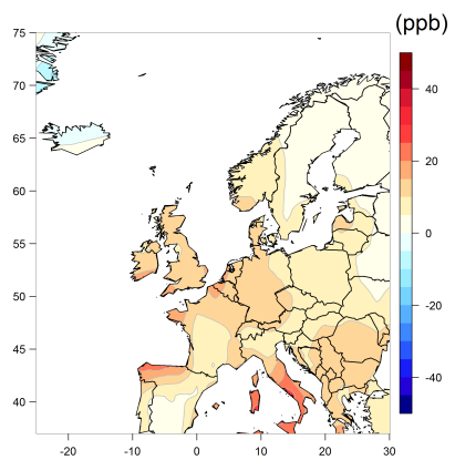
(f) MRIESM1r1
