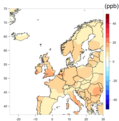
(c) GFDL-AM3
