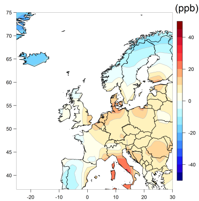
(a) CHASER
