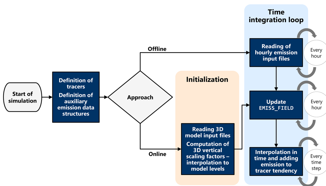
Figure 2. Flow chart for COSMO-GHG run-time processes both for the offline and the online approach. Blue rectangles are code parts. The simulation start point is represented by an oval.
